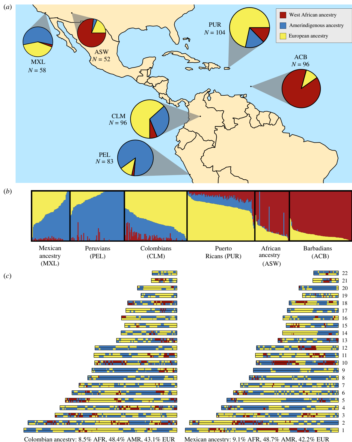
Figure 1. Ancestry in admixed populations varies at multiple genetic scales, with variance among individuals and within individual genomes. We show examples of global and local ancestry inferred from phased 1000 Genomes Project data for populations of the Americas and Caribbean. Global ancestry was estimated using unsupervised ADMIXTURE analysis, including additional populations of European (Iberians (IBS) and Tuscans in Italy (TSI)) and West African (Esan (ESN), Mandinka (GWD), Mende (MSL) and Yoruba (YRI)) ancestry for reference. We show (a) population-level and (b) individual-level estimates of global ancestry across Mexican ancestry (MXL), Peruvian (PEL), Colombian (CLM), Puerto Rican (PUR), African ancestry (ASW) and Barbadian (ACB) populations; barplots illustrating these estimates for K=3 were made using pong [6]. (c) Local ancestry as inferred by RFMix [7] for two example individuals (HG01149 and NA19776) who have similar global ancestry proportions, and belong to the CLM and MXL populations, respectively. For these analyses, we retained only SNPs marked 'PASS' and removed all individuals who were noted to have an up to third degree relative in the 1000 Genomes Project phase 3 pedigree file, leaving 998 individuals for analysis. We then filtered SNPs for missingness (greater than 5%) and low minor allele frequency (less than 1%) across all populations, and Hardy–Weinberg disequilibrium ( p -value < 0.000001 ) within populations. For our ADMIXTURE analyses, we also removed SNPs in linkage disequilibrium (using the PLINK command –indep-pairwise 50 10 0.1), which left 698 408 SNPs for analysis. We ran the ADMIXTURE algorithm for K=3 unsupervised using the default settings and a random seed. Pong identified a single mode across 30 replicates. To estimate local ancestry, we used the missingness, minor allele frequency and Hardy–Weinberg filtered phased genotype dataset. We designated individuals with high levels (over 99%) of global West African (AFR), Amerindigenous (AMR) and European (EUR) ancestry, as determined by our ADMIXTURE analysis, as reference groups for those respective ancestries. We ran RFMix v. 2.03 for the target Colombian and Mexican ancestry individuals using the HapMap GRCh37 genetic map lifted over to GRCh38, a maximum of two expectation-maximization iterations, and otherwise default parameters. (Online version in colour.)
